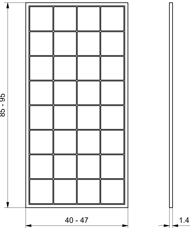
SOLAR PANEL SCALE 1 / 20
