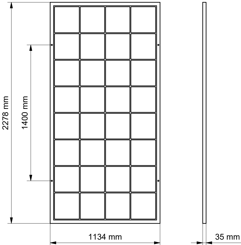
SOLAR PANEL SCALE 1 / 20
