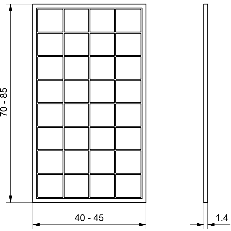
SOLAR PANEL SCALE 1 / 20
