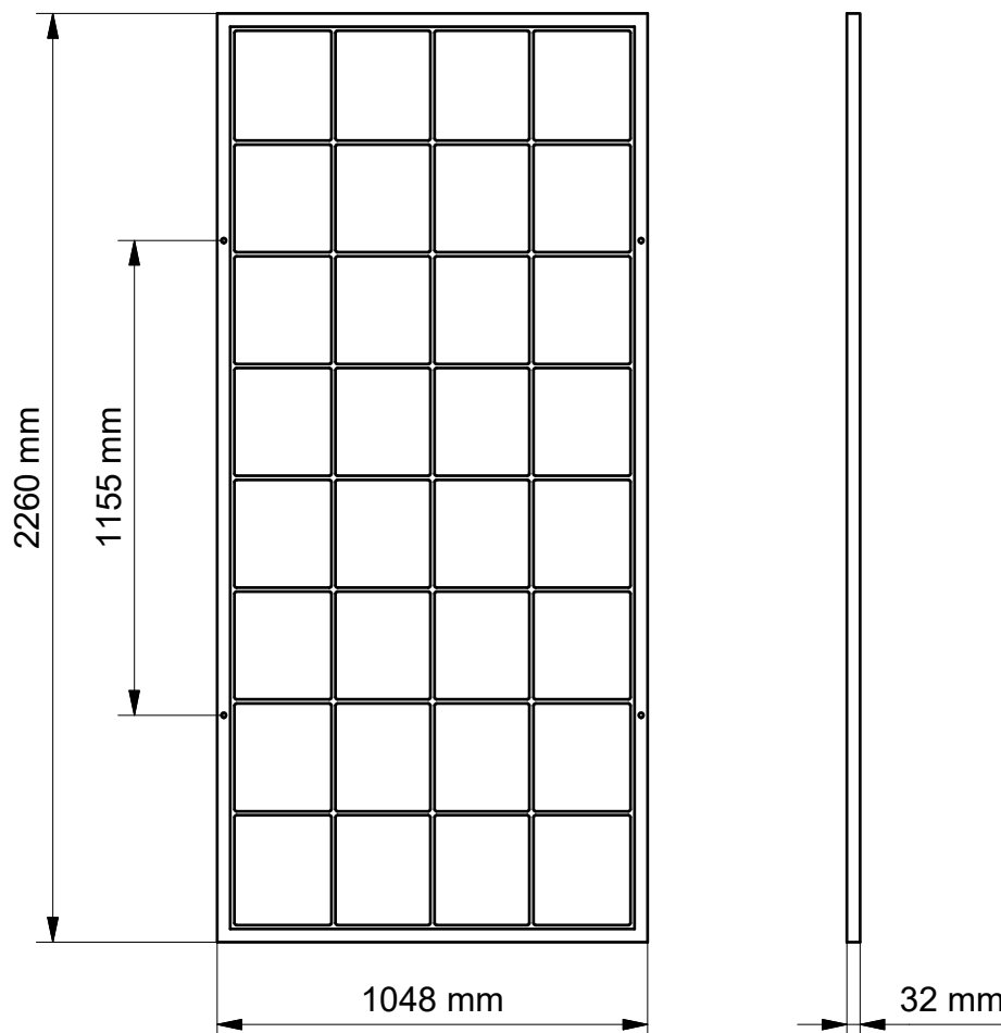
SOLAR PANEL SCALE 1 / 20
