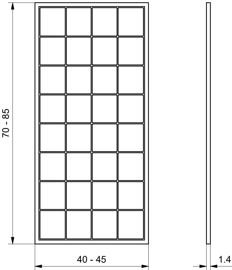
SOLAR PANEL SCALE 1 / 20
