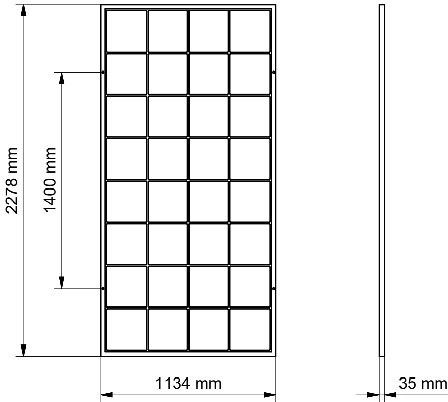
SOLAR PANEL SCALE 1 : 25
