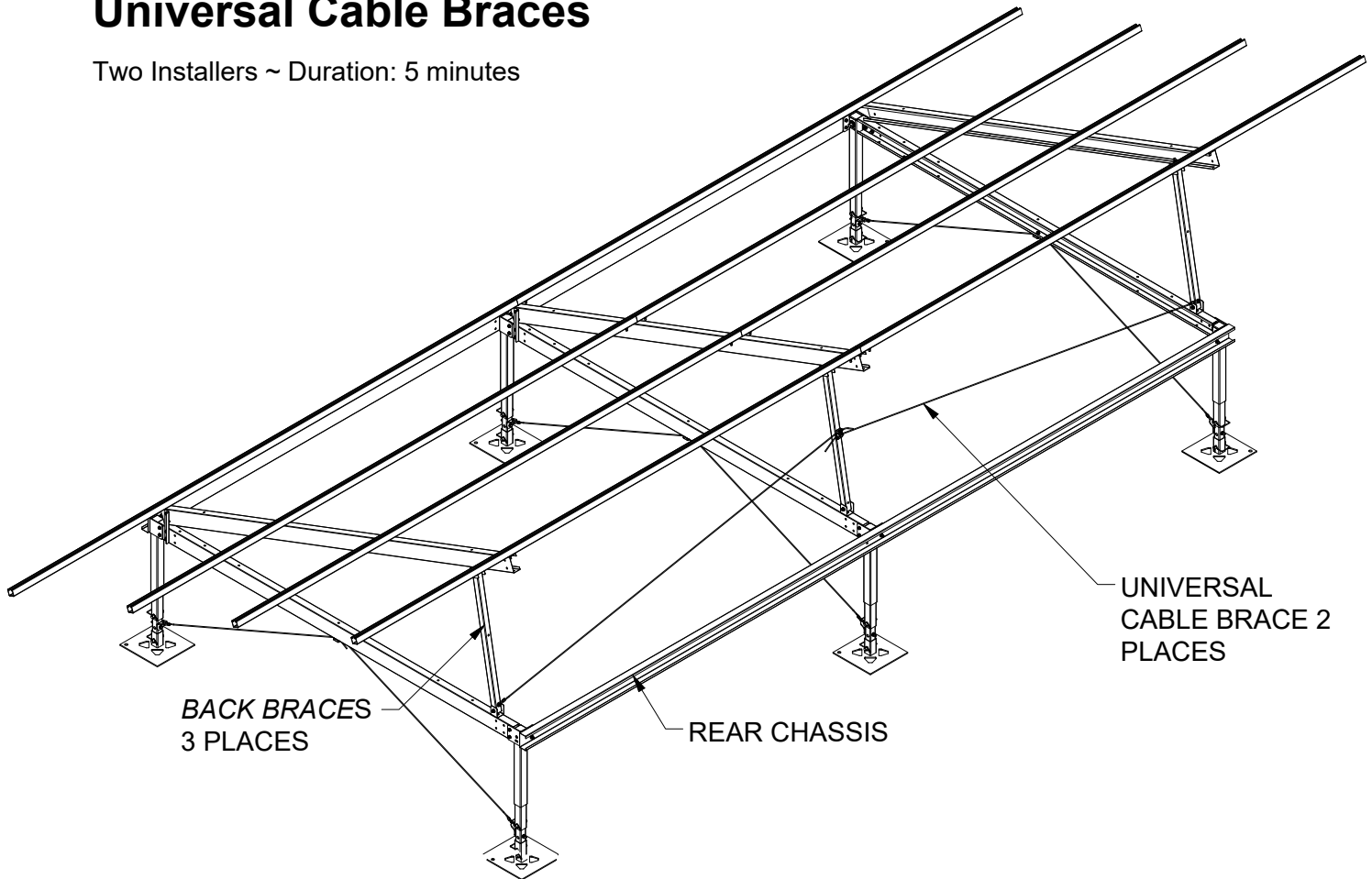
Figure 19: Cable Braces
