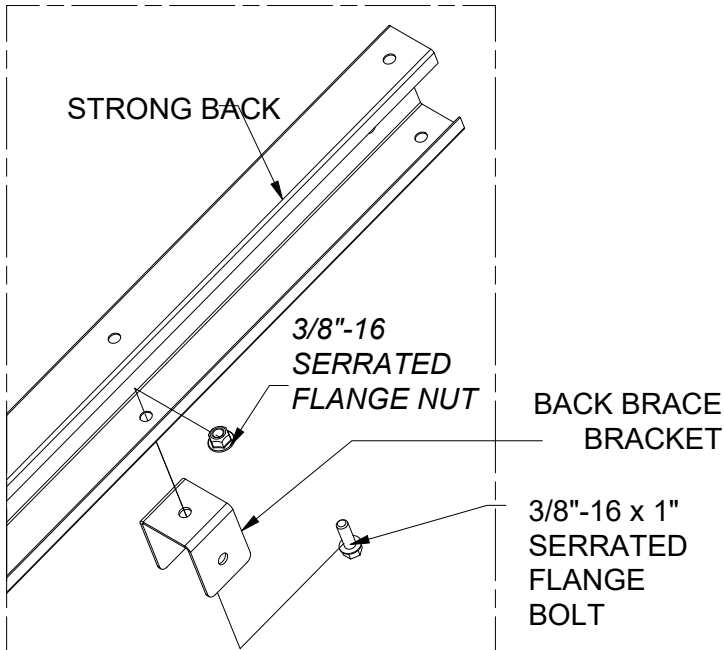
Figure 12: Back Brace Assembly (a)
