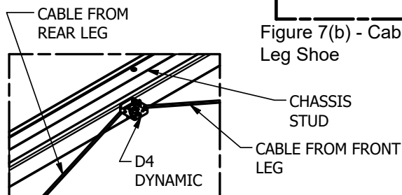
Figure 8(b) - Cable Routing Through the D4 Dynamic
