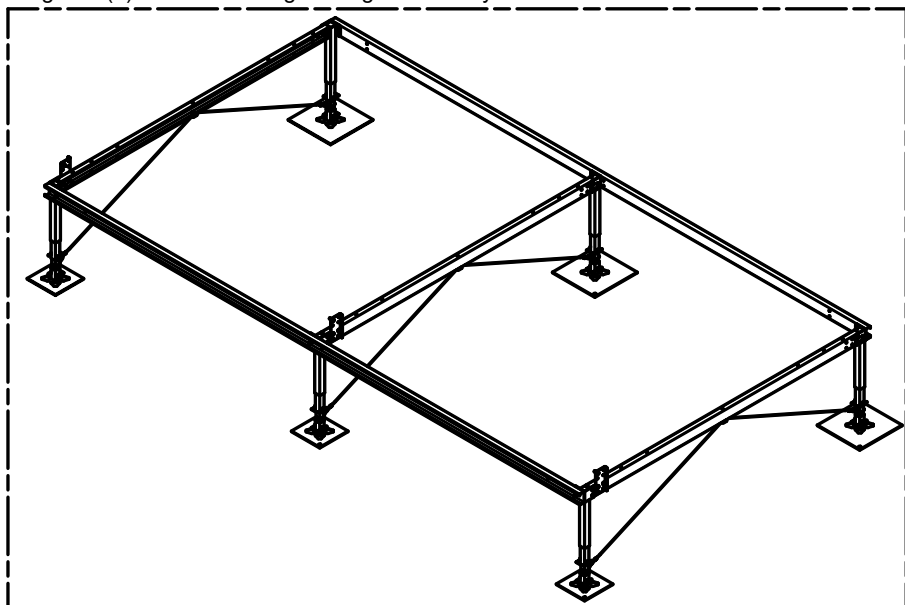
Figure 8(c) - General View "Chevron Cable Brace" - STD/HD/XHD
