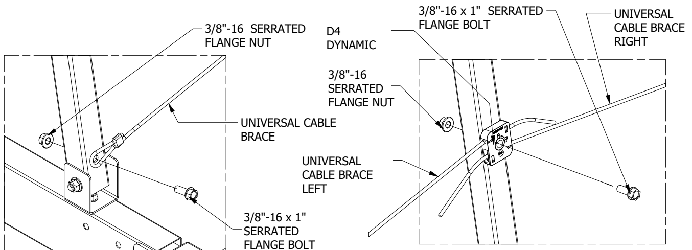
Figure 20: Universal Cable Brace Assembly (a)
