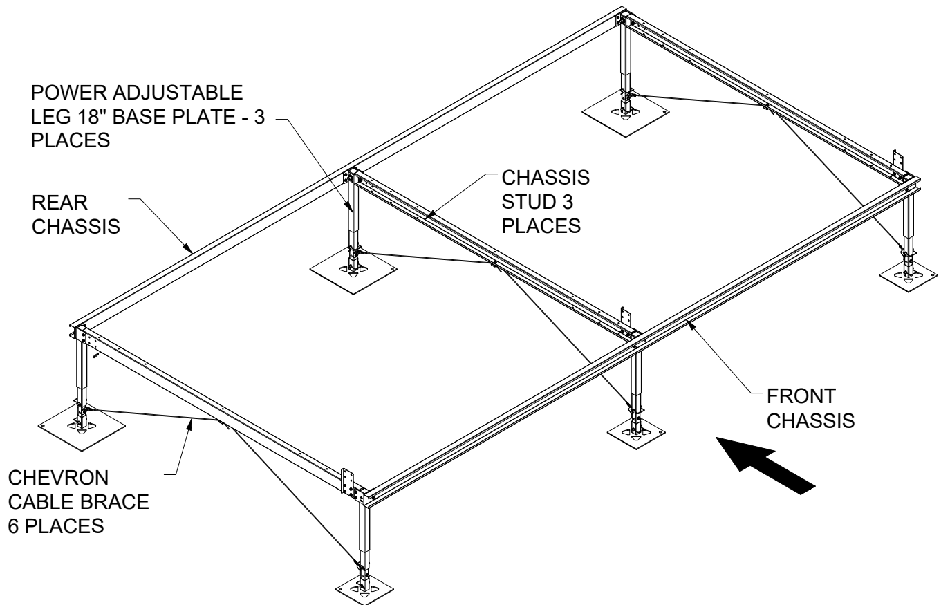
FIGURE 1(b): Osprey Chassis - STD/HD/XHD
