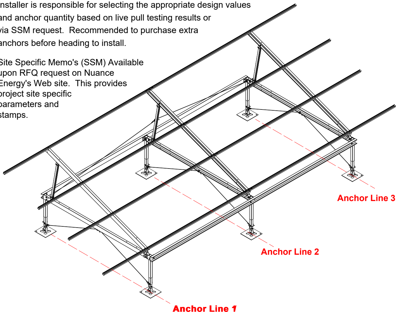
Figure 21: Earth Anchor Lines (a)
