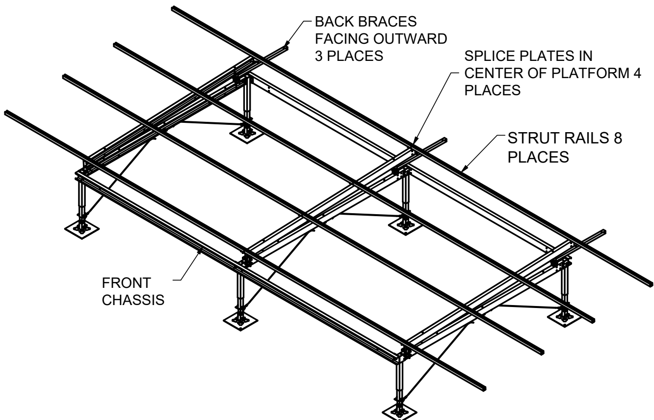
Figure 15: Strut Rails
