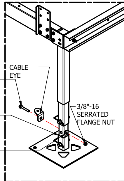
Figure 7(b) - Cable Eye Installation on Leg Shoe
