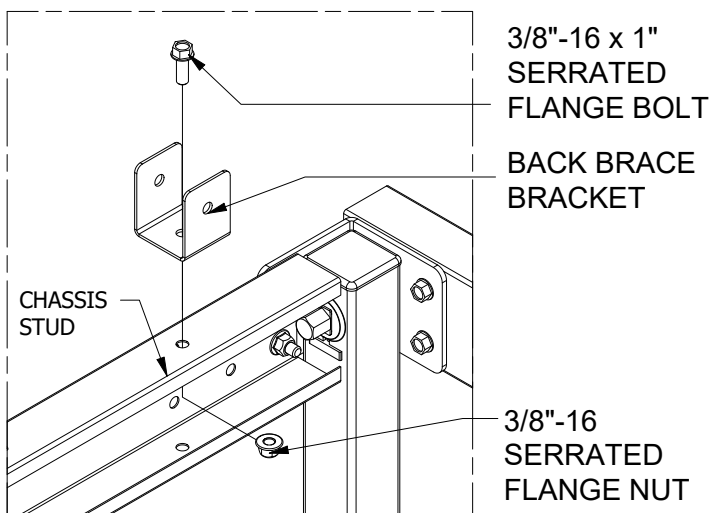
Figure 12: Back Brace Assembly (b)
