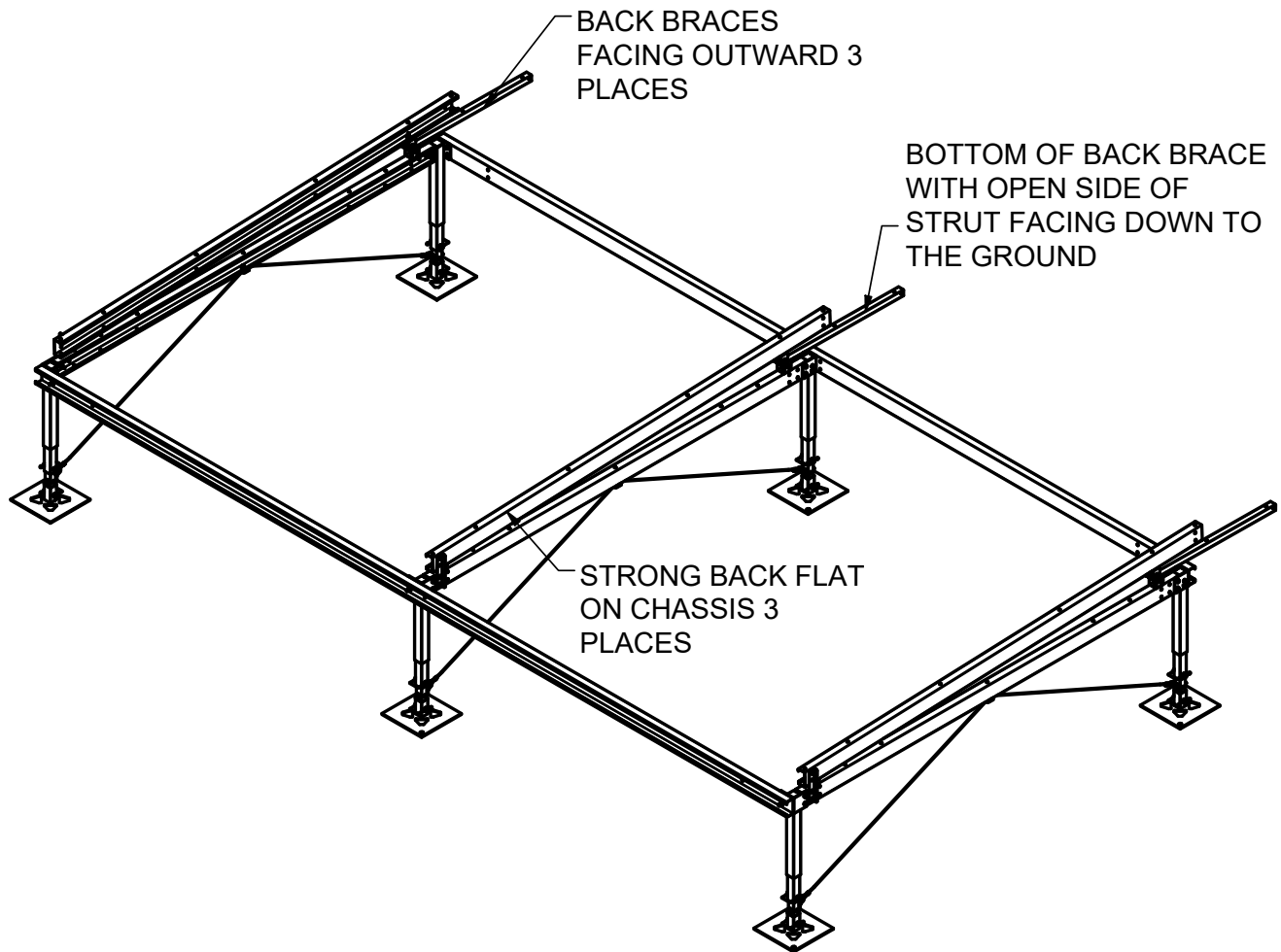
Figure 14: Alternate Back Brace Installation prior to installing Strut Rails.
