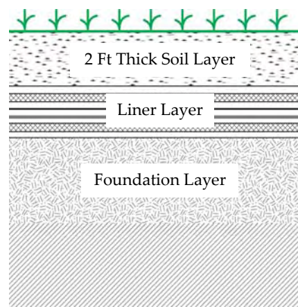
Figure 6: Typical RCRA Landfill Cover
