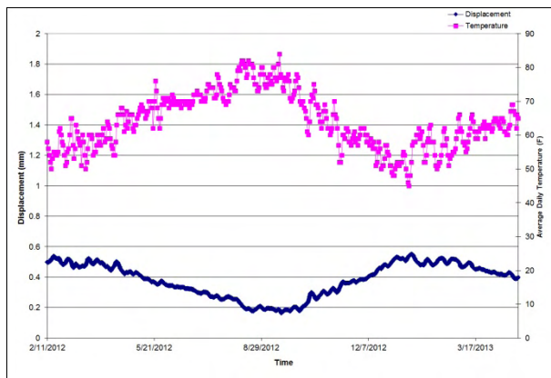
Figure 11: Time vs Displacement and Temp
