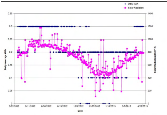
Figure 14: Time vs kW and Daily Maximum Solar Radiation
