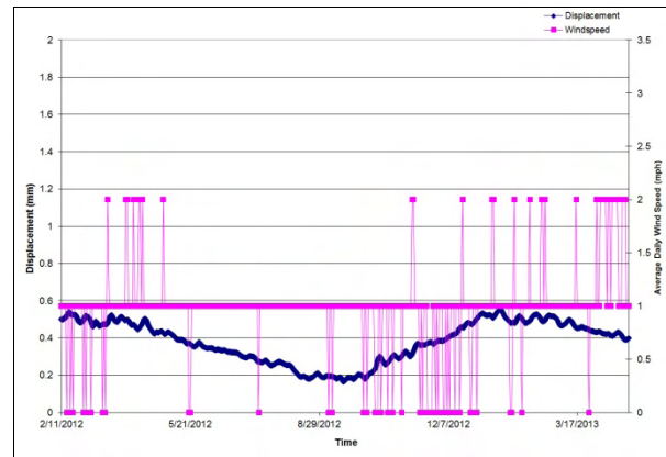
Figure 12: Time vs Displacement and Wind Speed
