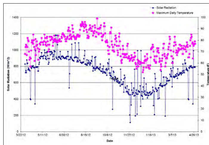
Figure 13: Time vs Maximum Daily Solar Radiation and Maximum Daily Temperature
