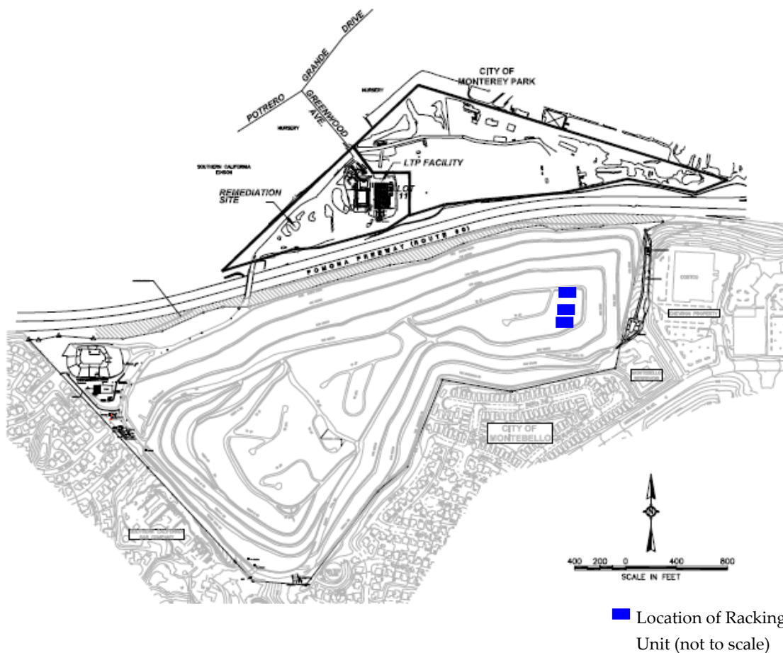
Figure 4: Location of Solar Racking Units at Site
