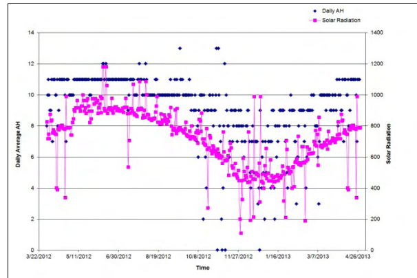
Figure 15: Time vs Ampere and Daily Maximum Solar Radiation
