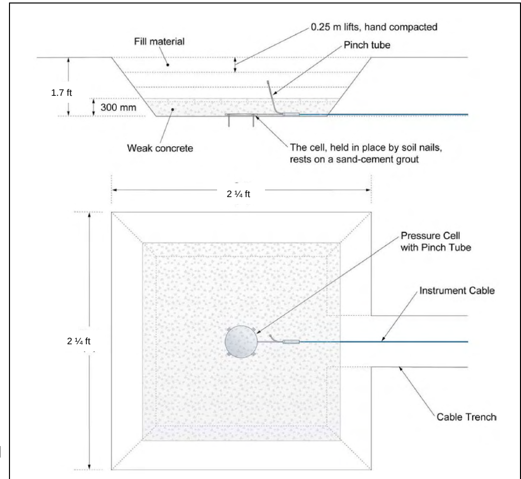
VW Earth Pressure / Load Cell Schematic Diagram and Installation Detail
