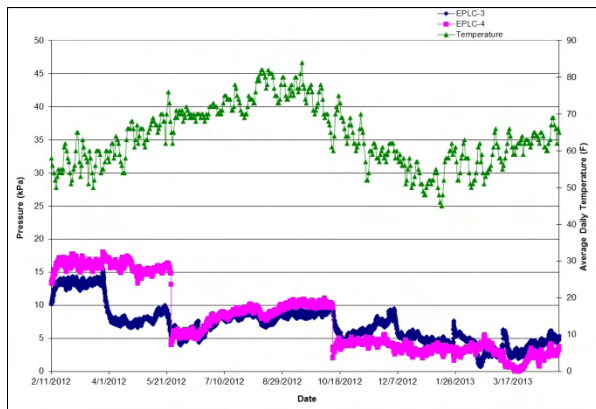
Figure 9: Time vs Load and Temperature at EPLC-3 and EPLC-4
