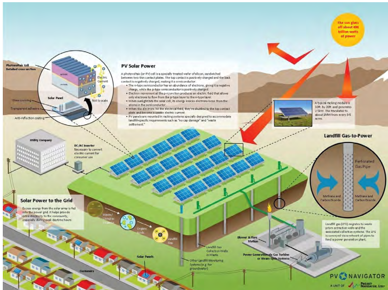
Figure 1: Conceptual Design of a PV Solar Facility on a Closed Landfill Located in Urban Area
