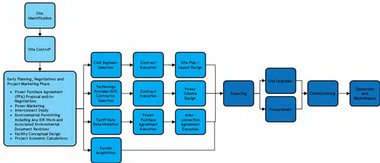
Figure 2: Flow Diagram Outlining Steps the Process for the Development a Solar Facility
