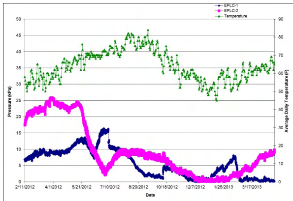
Figure 7: Time vs Load and Temperature at EPLC-1 and EPLC-2
