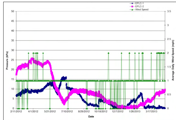
Figure 8: Time vs Load and Wind Speed at EPLC-1 and EPLC-2
