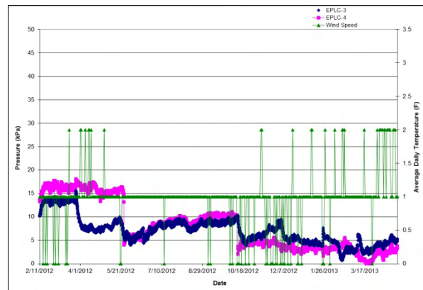
Figure 10: Time vs Load and Wind Speed at EPLC-3 and EPLC-4
